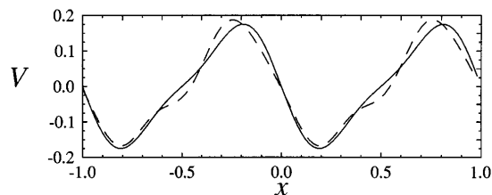
FIG. 1. Shape of the two ratchet potentials V_2(x) (solid) and V_3(x) (dashed) used in this work.
