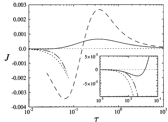
FIG. 4. The current reversal in V_3(x) is depicted for D = 0.05 and Q(\tau) = Q = 0.025 : Numerical results (solid line) are compared to GUCNA (dash-dotted line), small- \tau (dotted line), and small- \gamma (dashed line) theory. The inset gives a magnification of the behavior at small \tau .
